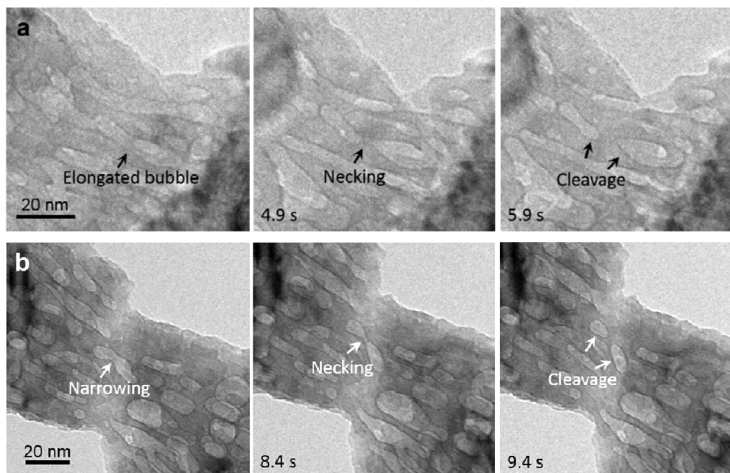
Figure S1. Fragmentation of helium bubbles under plastic strain. (a) Bubble fragmentation under multiple shear; (b) Bubble fragmentation process under single shear.
