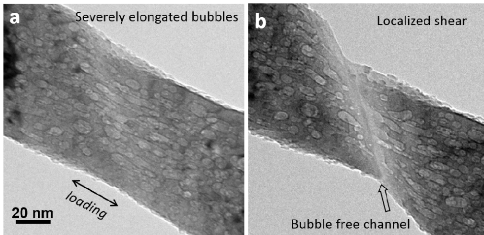
Figure S4. Bubble free zone formed via bubble cleavage at the final fracture stage of helium bubbled copper. (a) Severely elongated bubbles after tensile deformation; (b) Bubble fragmentation leads to the formation of bubble free zone before the final fracture.
