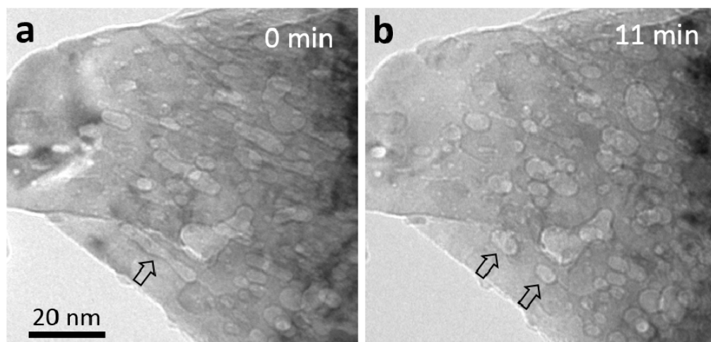
Figure S2. Rayleigh instability induced fragmentation of the elongated bubbles during aging in vacuum. (a) The elongated bubble post to unloading as indicated by the black arrow. (b) Two elliptic bubbles fragmenting from the elongated bubble after 11 mins aging.
